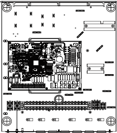
Internal View
